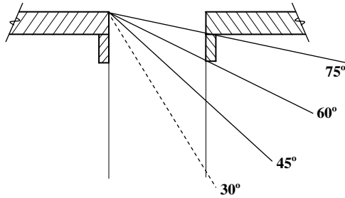
Fig. 2. Horizontal and Vertical Shading Device (Designed by Authors)
