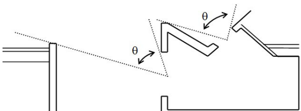
Fig. 3. Angle of q , which defines visible sky from centre of window/rooflight
