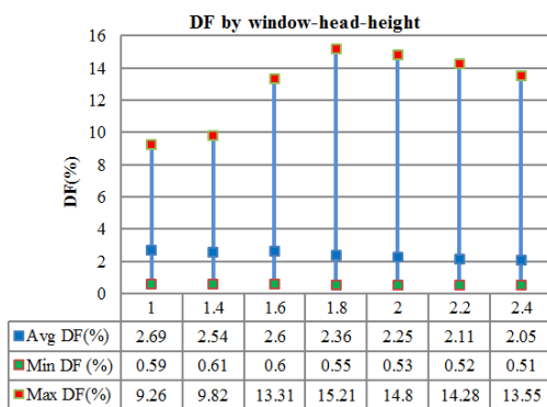
Fig. 8 DF by changing window-head-height
