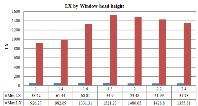
Fig. 10 Minimum and maximum illuminance levels by changing window-head –height
