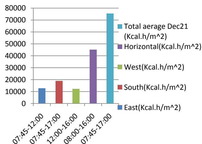
Fig. 11 Radiated solar energy on every surface
