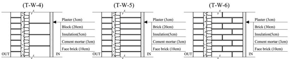
Figure 2: Details of insulated exterior walls' structures.
