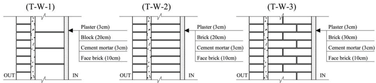
Figure 1: Details of none-insulated exterior walls' structures.
